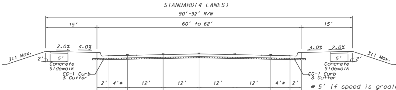
SECONDARY ARTERIAL W/O PARKING
