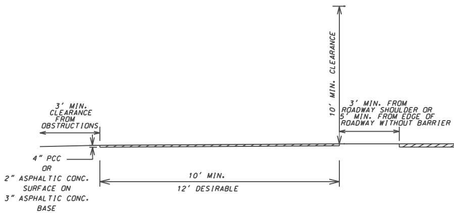
TYPICAL BIKE TRAIL SECTION
