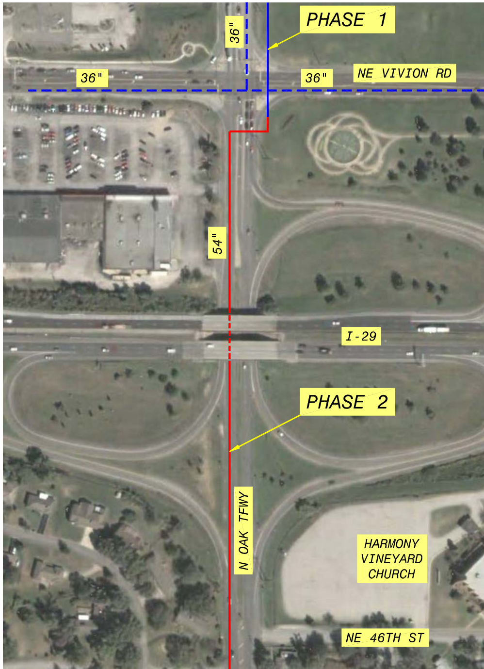
I-29 INTERCHANGE
